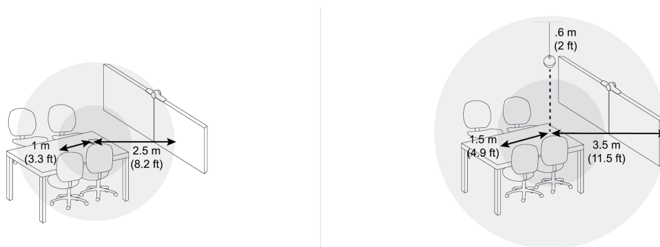
Figure 2. 2 IP Table or 2 IP Ceiling Microphone Layout
