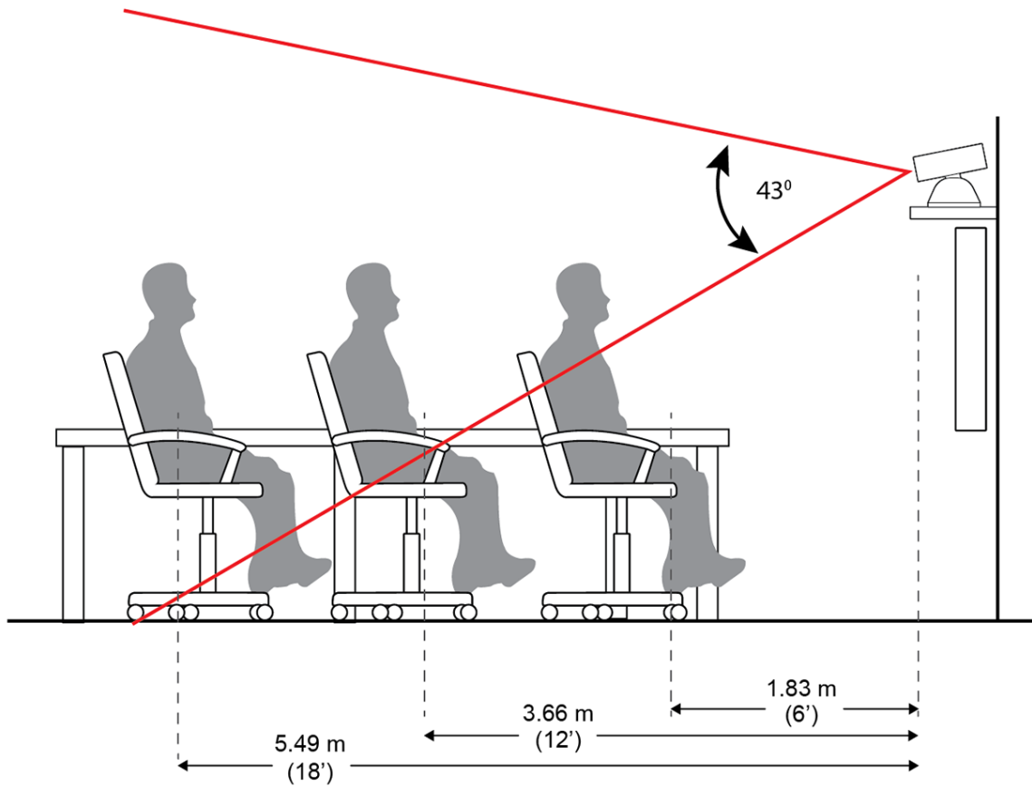
Figure 2. Poly Studio E60 HFOV with the first seat approximately 1 m (3.3 ft.) feet from the camera
