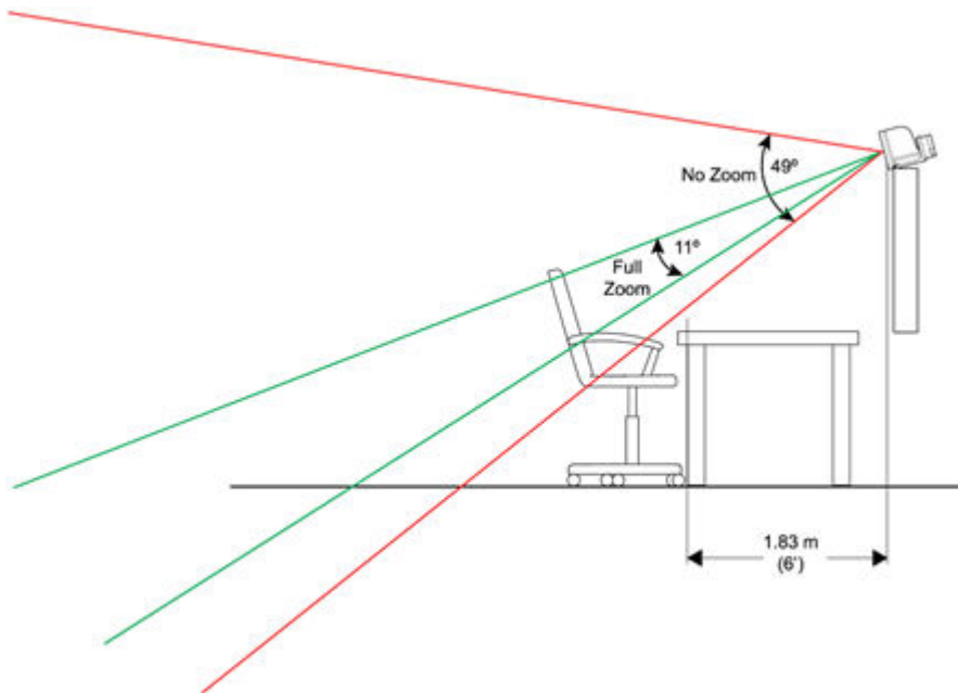
Poly Studio E70 in a modest tilt position
