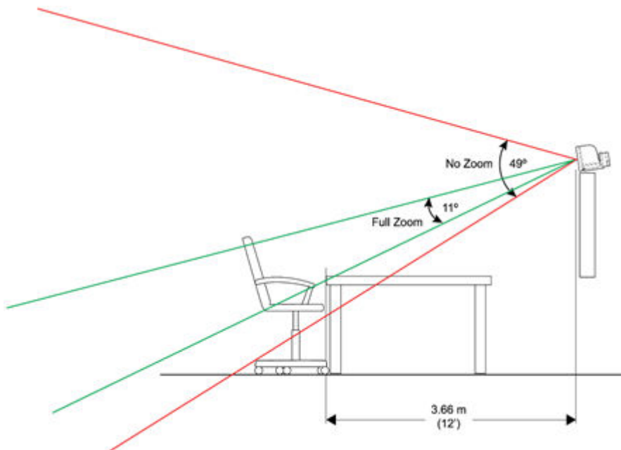
Poly Studio E70 in a level position
