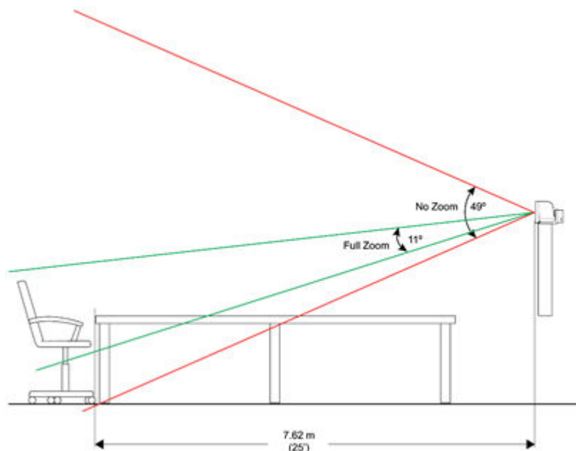
Poly Studio E70 with Poly DirectorAI Perimeter Configured
